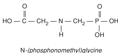
Figure 1 Glyphosate
